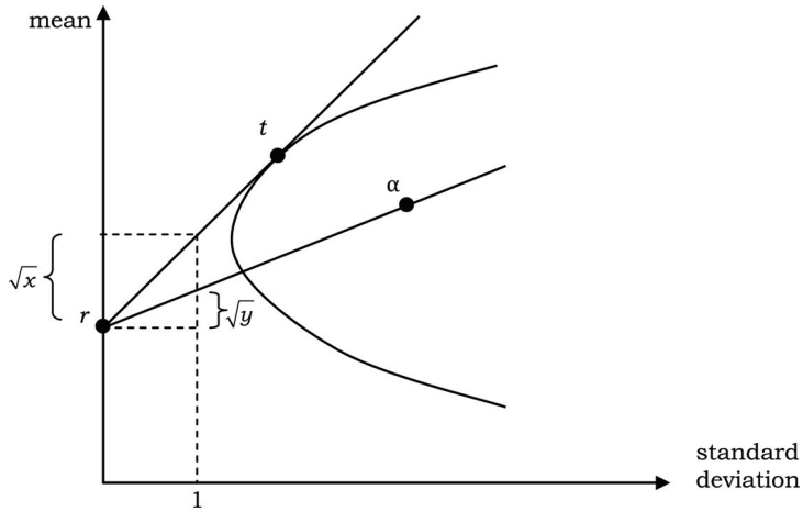
FIGURE 2 LIKELIHOOD RATIO TEST STATISTIC OF ROSS
